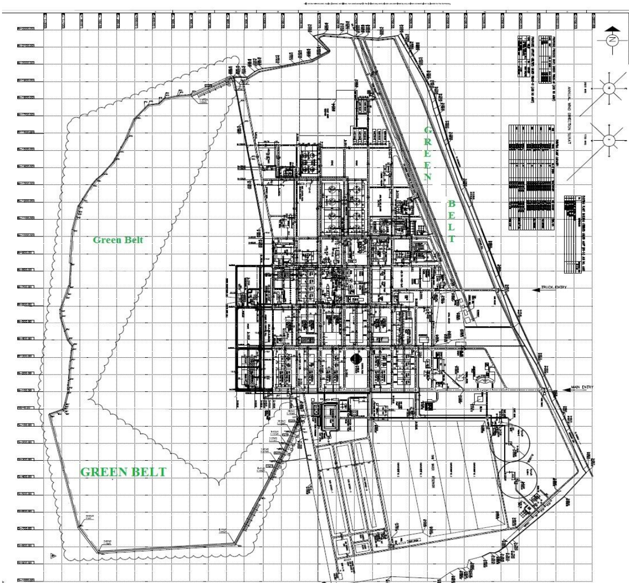
Annexure-4: GREEN BELT ONGC HAZIRA PLANT LAYOUT
